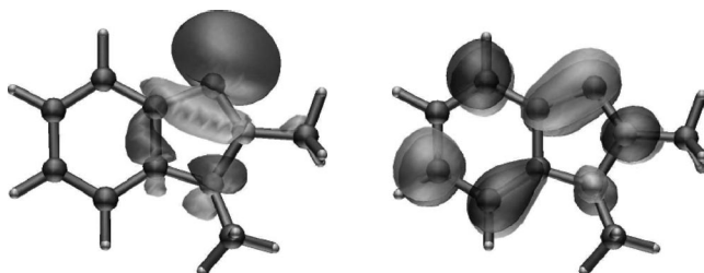
Figure 2. HOMO (left) and LUMO (right) of 2 .
