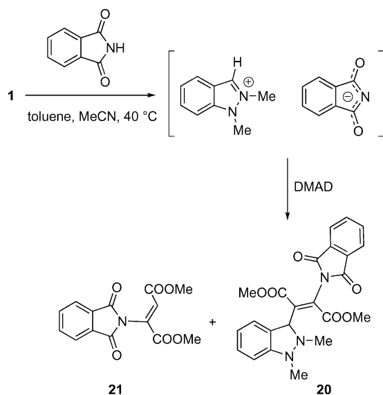
Scheme 13.
