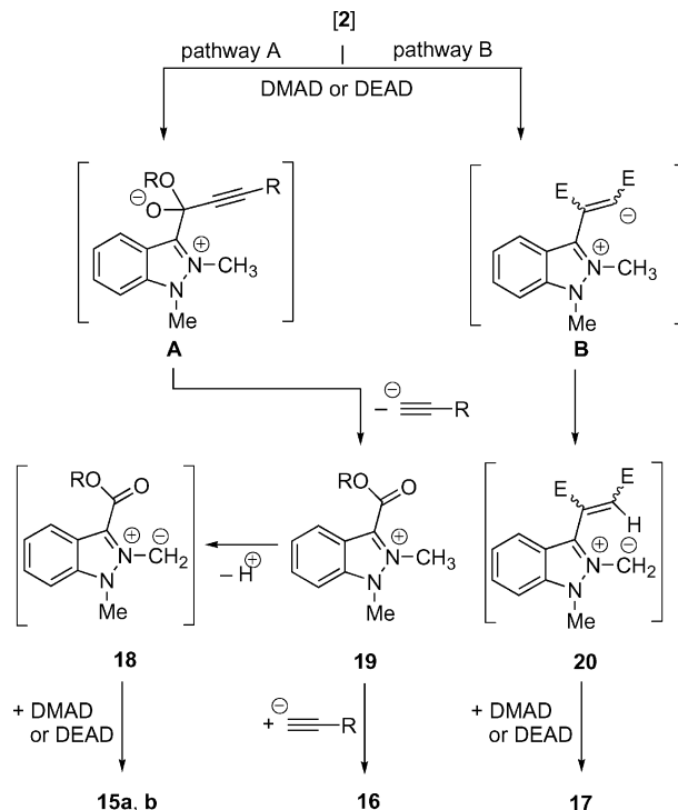
Scheme 11.
