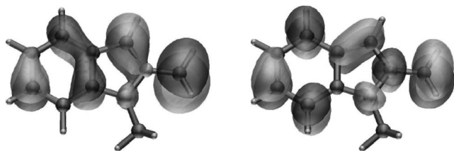
Figure 3. HOMO (left) and LUMO (right) of ylide 12a .
