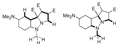
Figure 4. Some characteristic couplings in the HMBC measurements of 15d .
