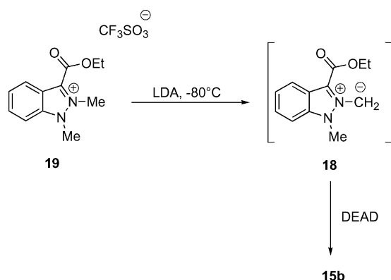
Scheme 12.
