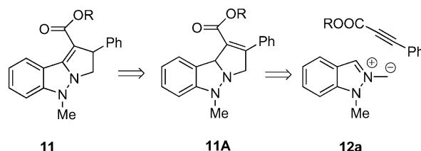
Figure 1. Retrosynthesis of ring system 11 .
